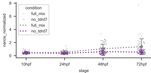
Normalized nuclear fluorescence across stages
