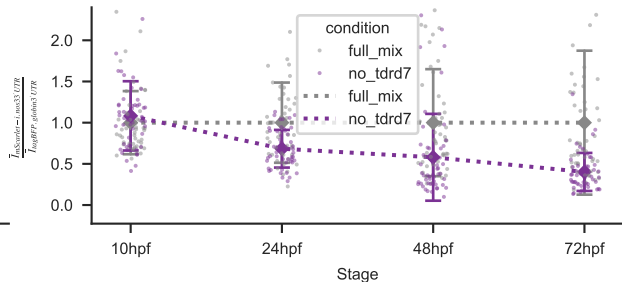
Normalized nuclear fluorescence across stages
