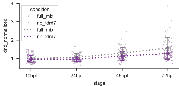
Normalized mean nuclear fluorescence across stages
