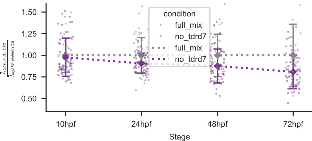
Normalized mean nuclear fluorescence across stages
