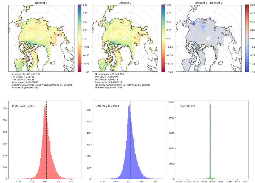
Figure 6: gridded maps (top) and histograms (bottom) of Arctic sea ice heights (ssh_flag = 0) from ATL07 during March 2019. Dataset 1: rel004, Dataset 2: test rel005. Note the difference in regions where the PODPPD flag = 4. Due to the change in along-track distance/spatial sampling during off-pointing scans it is challenging to determine any underlying bias in these data.
