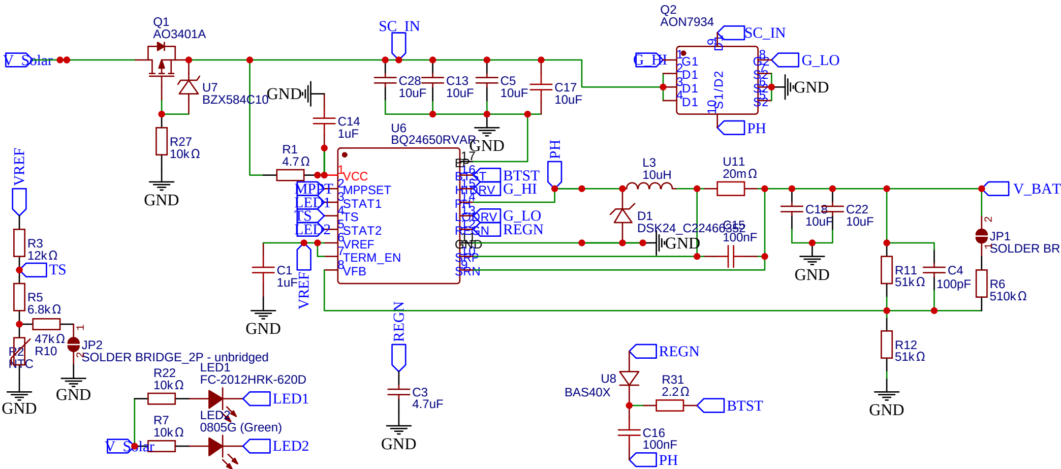
MPPT Solar Battery Charger 2A max charging current
