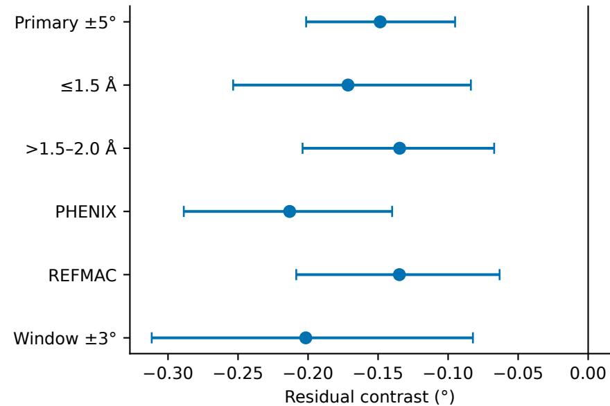
D \alpha robustness
