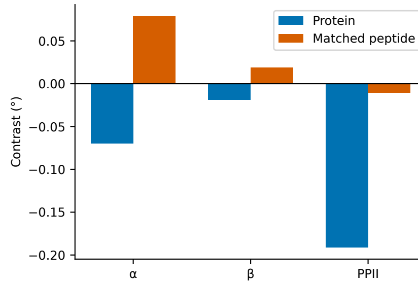
B Protein versus matched peptide
