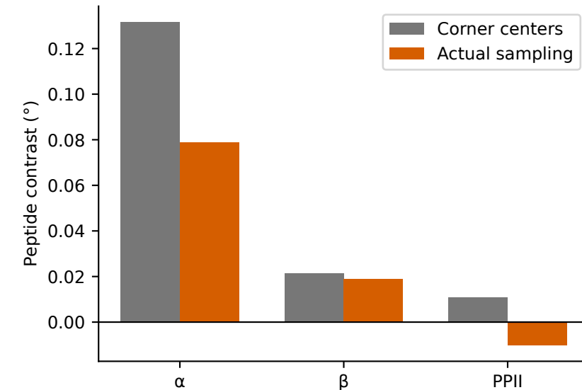
F Matching changes the prediction
