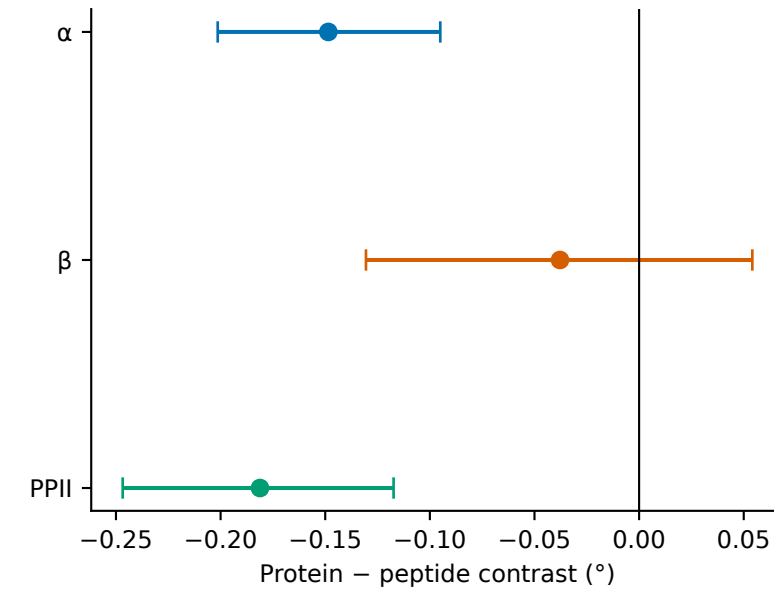
C Magnitude of the gap
