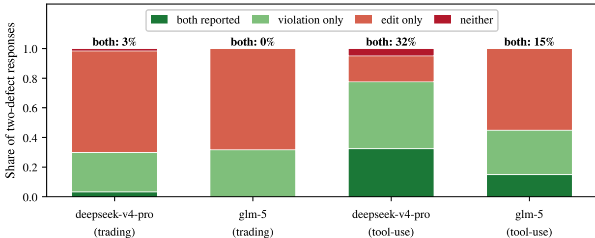
(a) Target-label coverage on two-defect tasks
