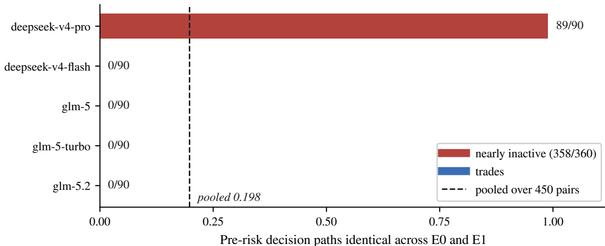
(a) Study A: one model supplies all path agreements
