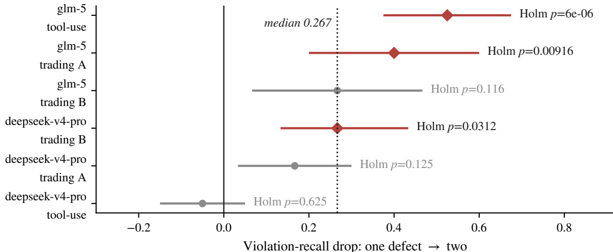
(b) Study B: six cells, three survive Holm
