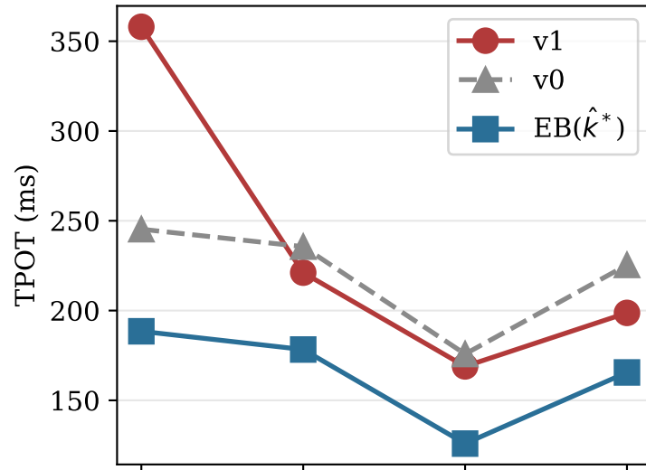
Time per Output Token ( \downarrow better)
