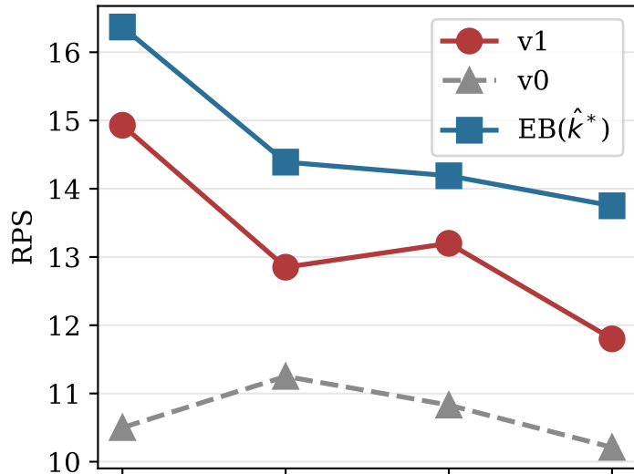
Throughput ( \uparrow better)
