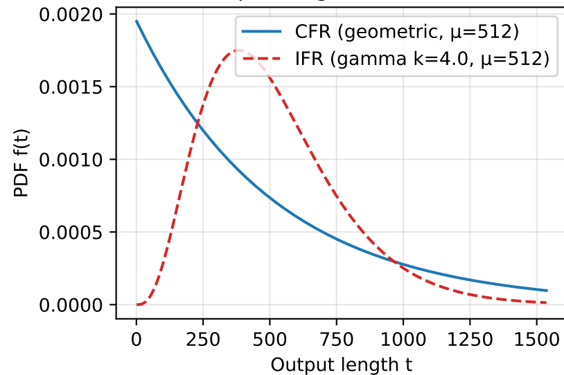
Output length distribution
