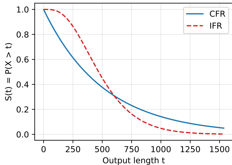
Survival function
