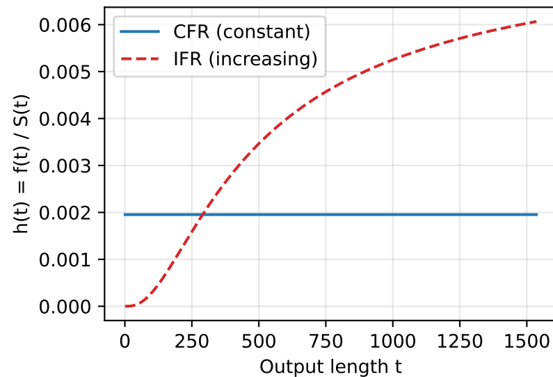
Hazard rate
