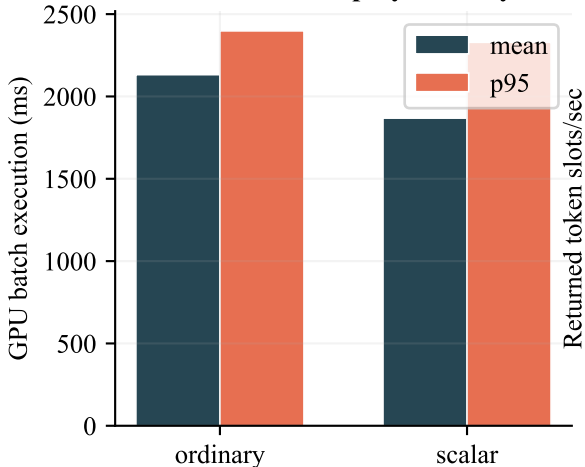
Real Batch Replay Latency
