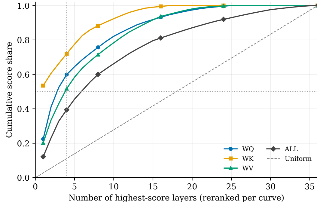
Positive mean \Delta\text{NLL}
