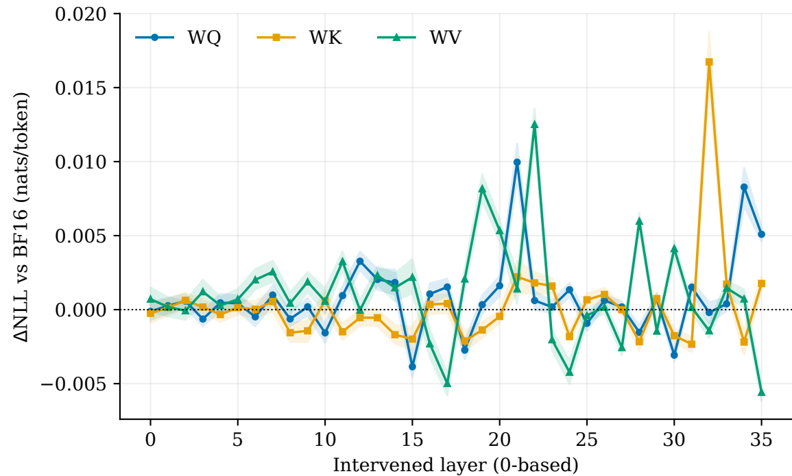
Qwen3-4B: one projection weight at RTN4; 64 blocks \times 2048 predictions Bands: exploratory paired-block 95% CIs (not multiplicity-adjusted)
