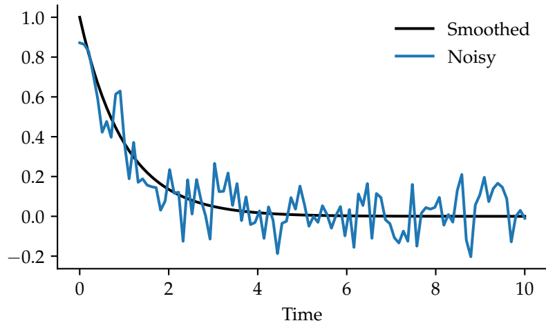
Loss
