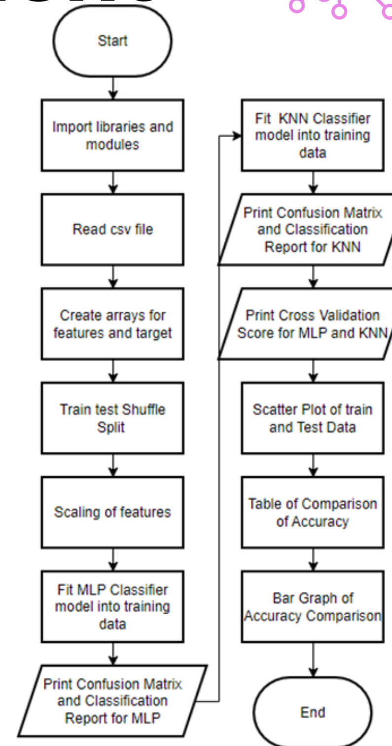
Flowchart for Training ML Models
