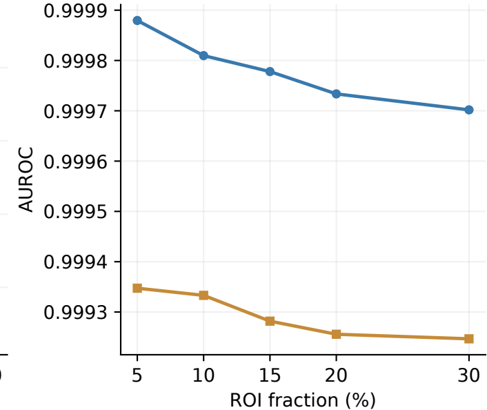
Replay-Attack
