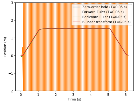
Figure E.25: Sampling methods for system simulation with T = 0.05 s
