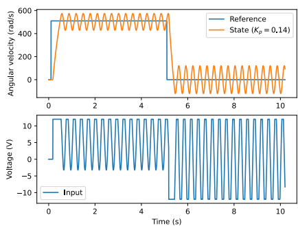
Figure B.5: Flywheel response at 1 ms sample period with 80 ms of output lag
