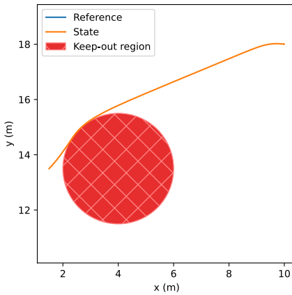
Figure 17.5: Differential drive MPC x-y plot
