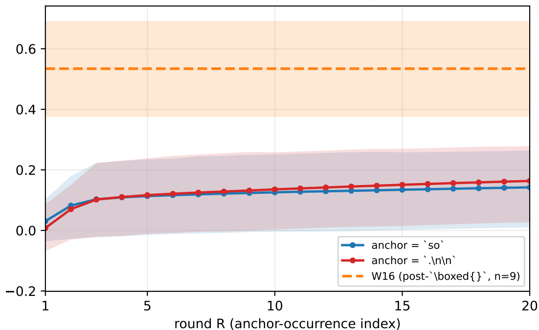
brumo25 (round-R n=8)
