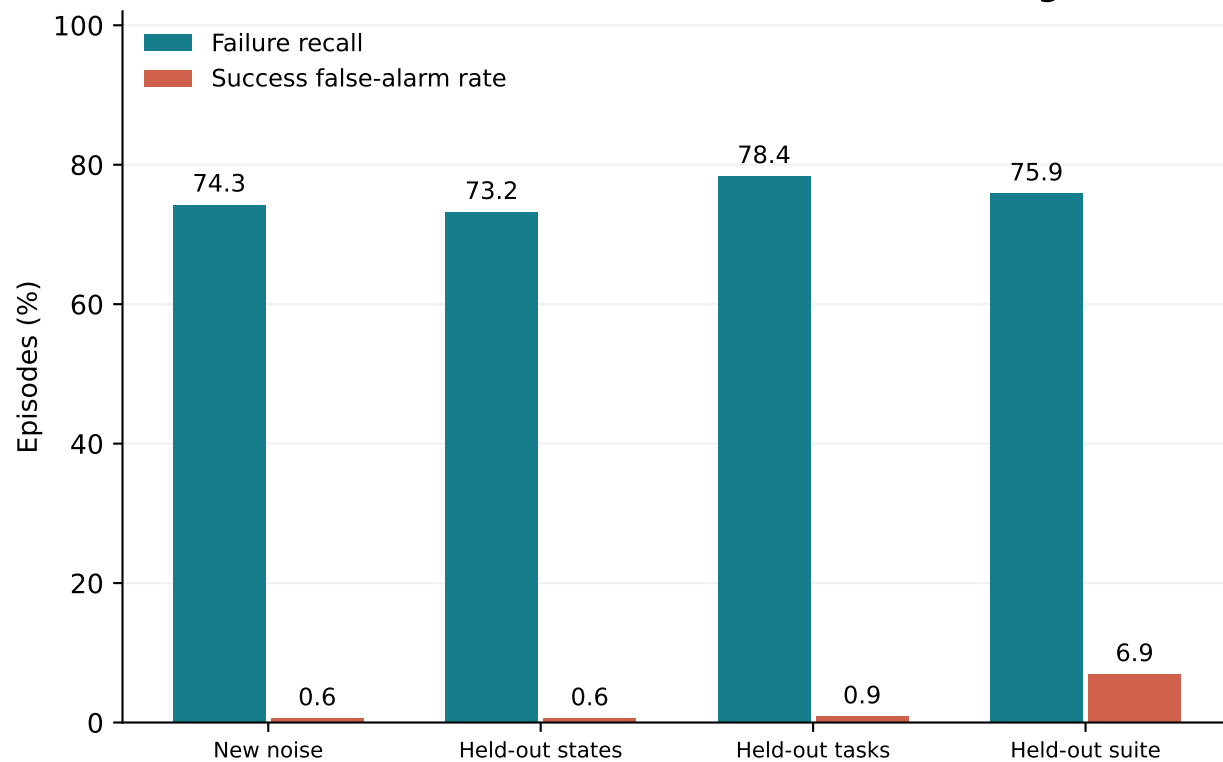
A. Fixed 3% unlabeled reference alarm budget
