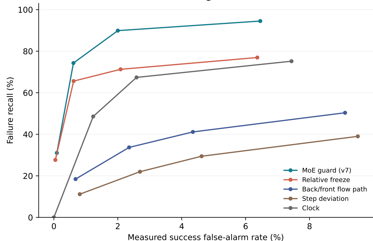
D. Release of failed goal subject (n=206)
