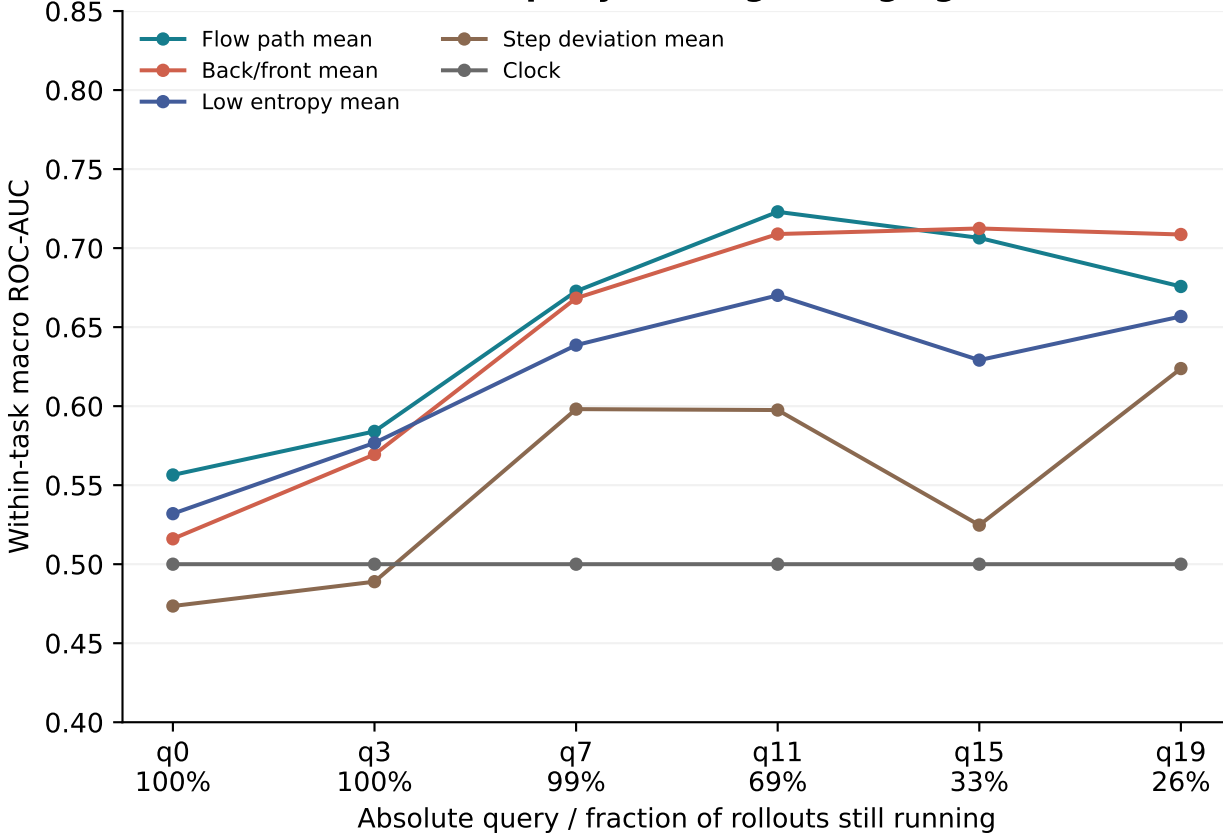
C. Causal fixed-query ranking; changing risk sets
