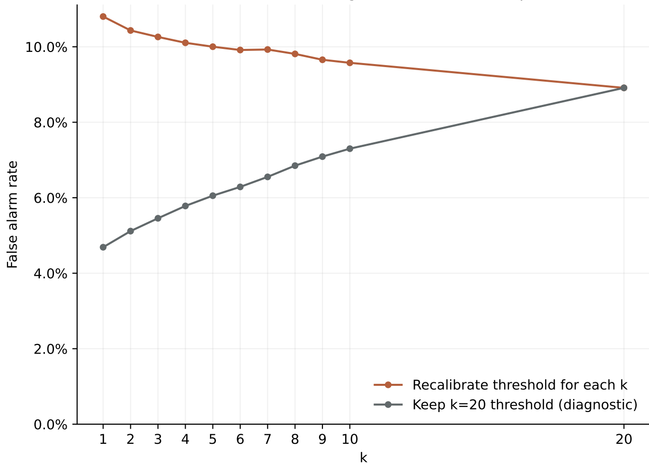
Euclidean: score shrinkage and threshold adaptation
