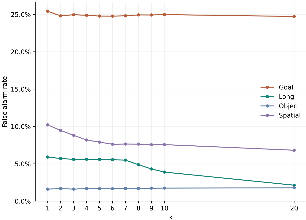
Euclidean false alarms by held-out suite
