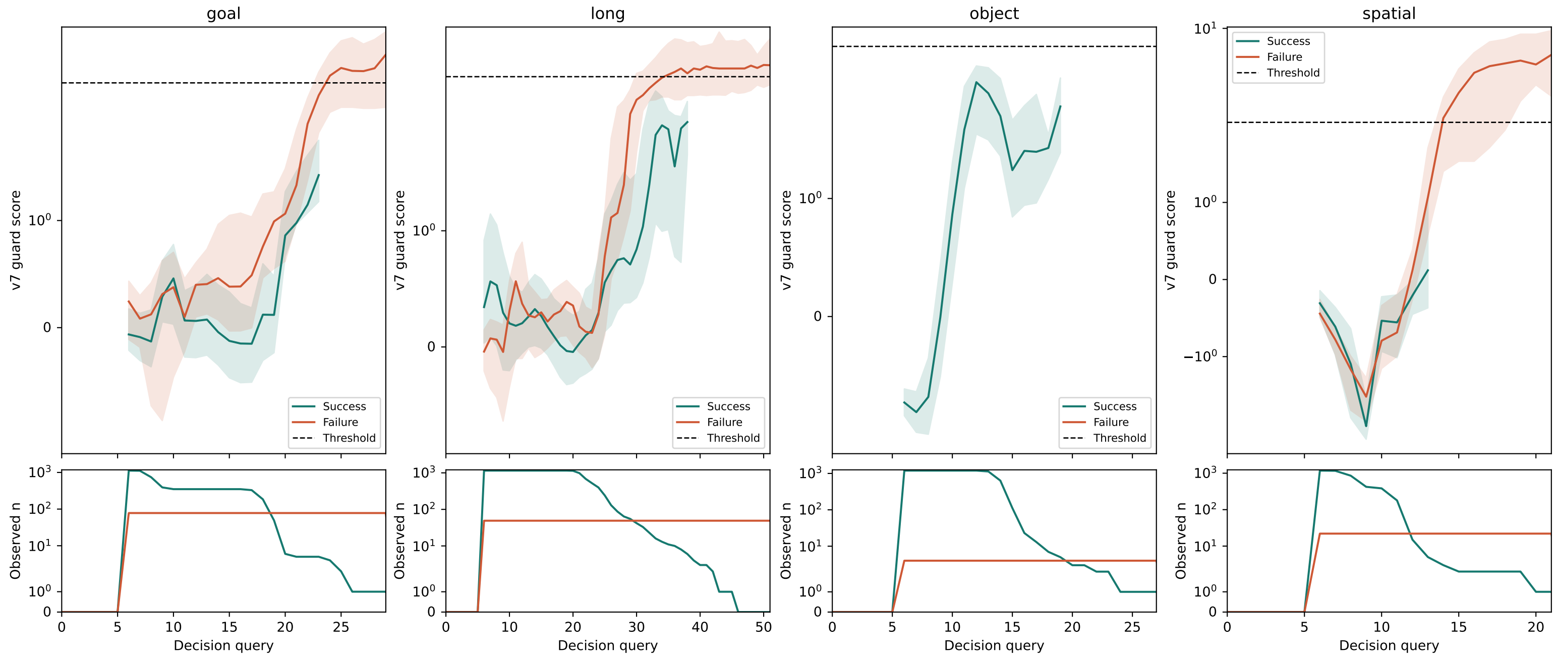
v7 risk over the observed prefix: first task split, unseen tasks
