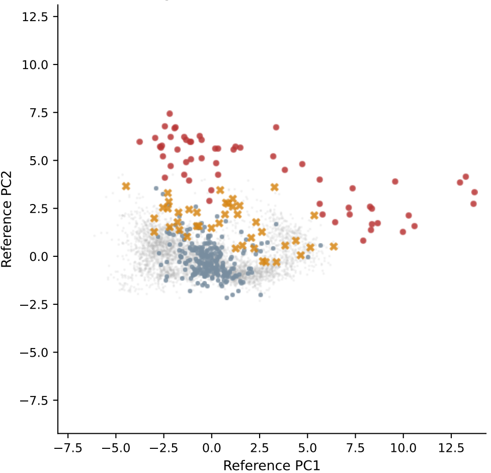
Current threshold decisions Orange X: 10D exceeds, 2D does not
