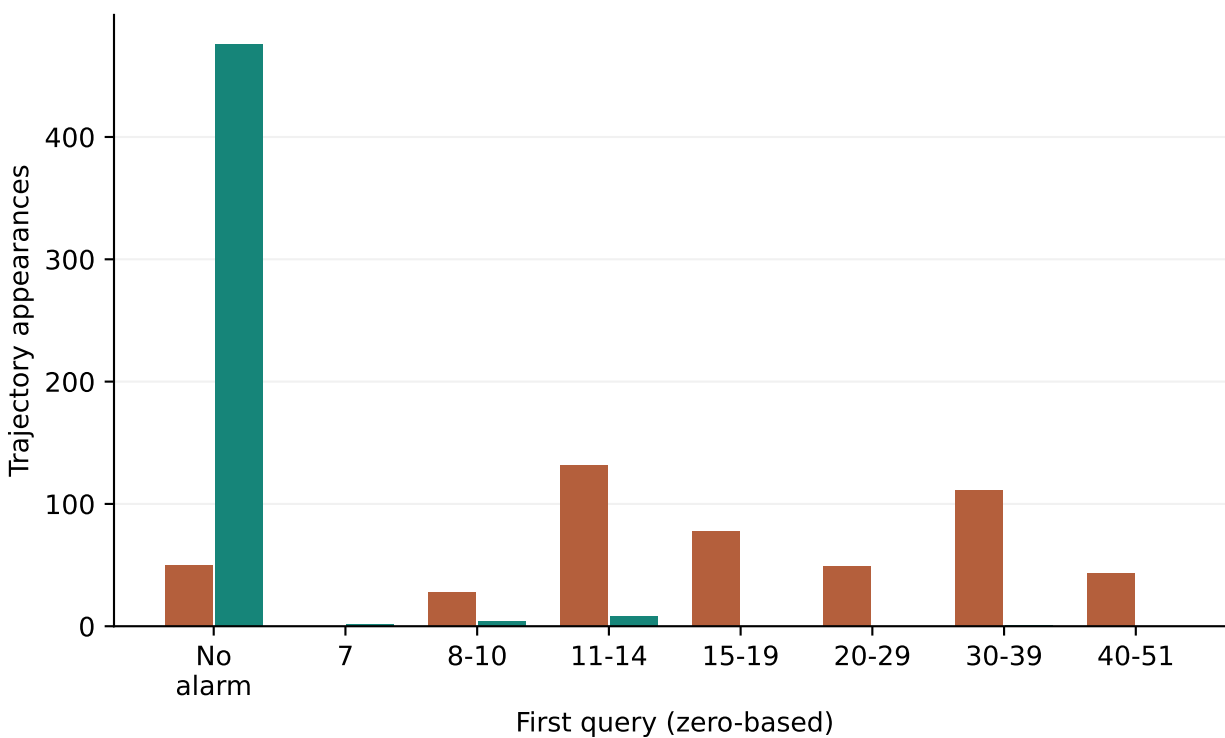
Unseen failures: first alarm distribution
