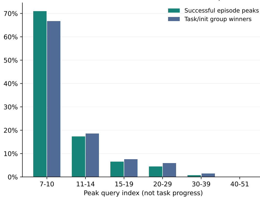
Where successful calibration cosine scores peak
