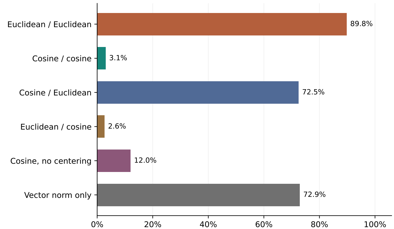
Same q33: reference direction and magnitude
