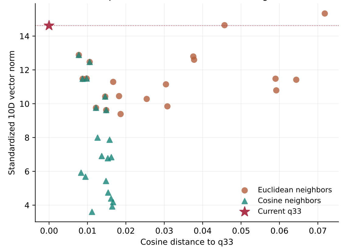
Same q33: reference direction and magnitude
