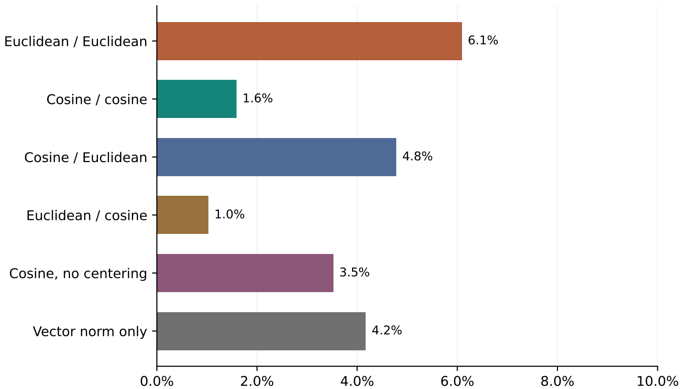
Where successful calibration cosine scores peak
