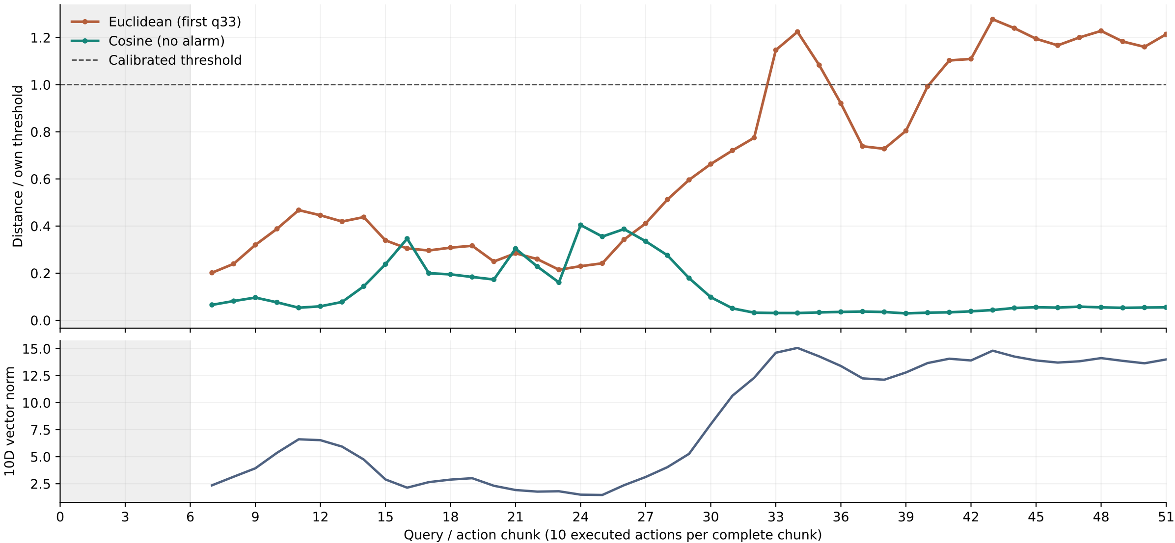
Same recorded trajectory: LIBERO-Long, episode 223 (52 chunks)
