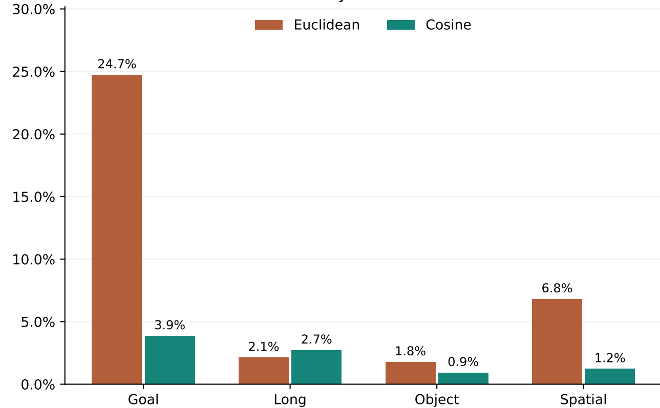
False alarms by held-out task suite
