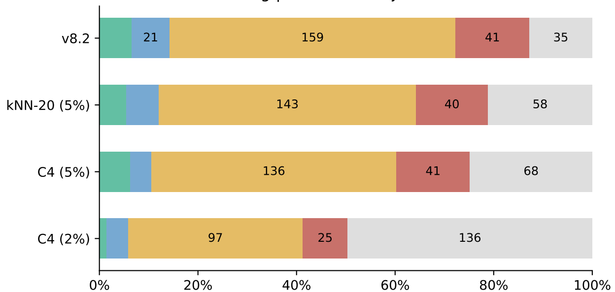
Long | 274 failed trajectories
