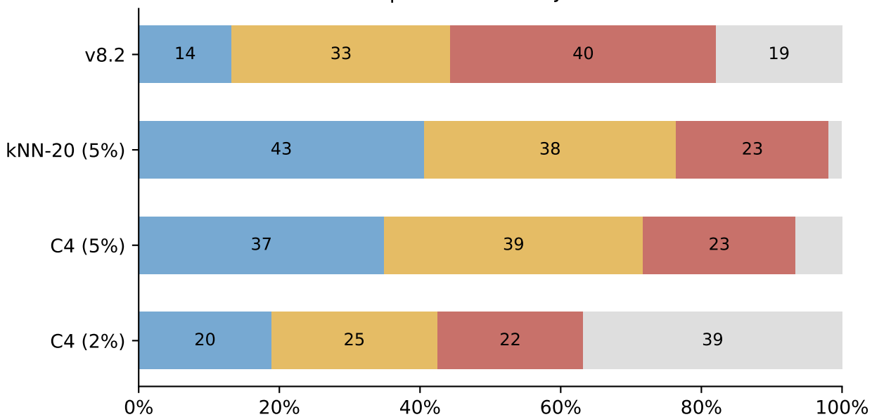
Goal | 106 failed trajectories
