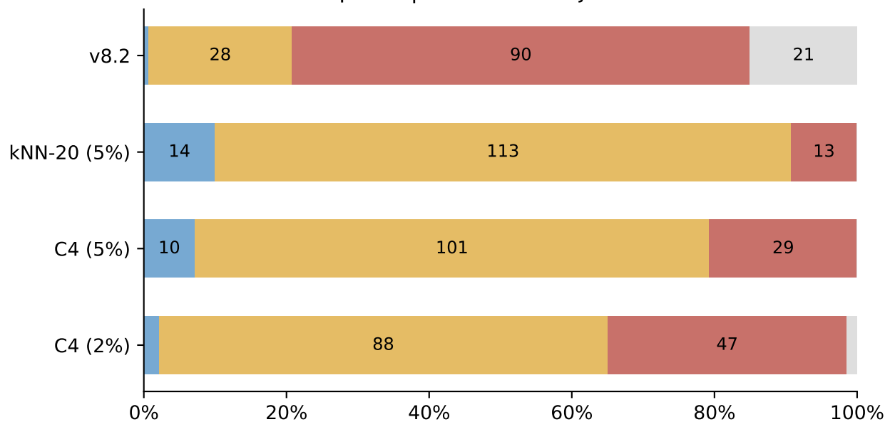
Spatial | 140 failed trajectories
