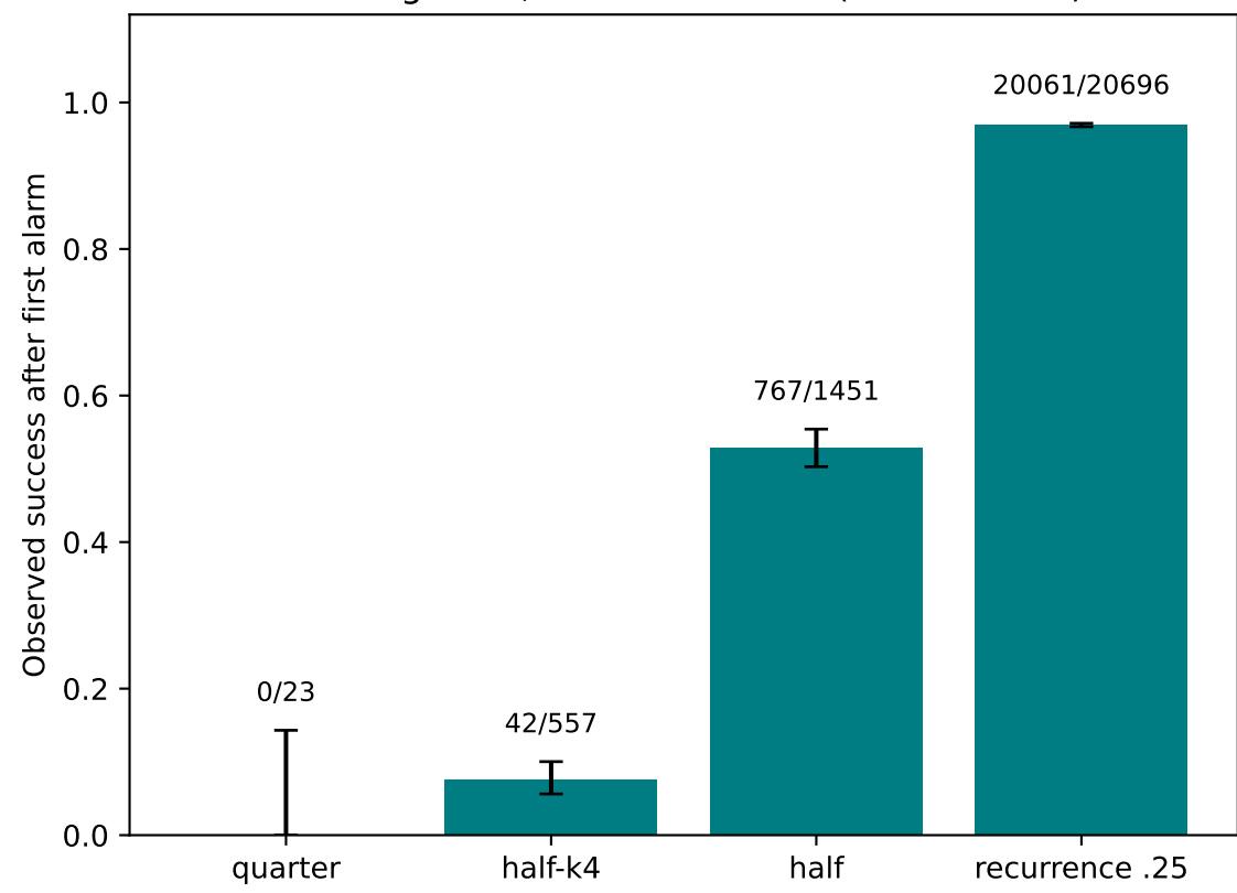
Existing rules; Wilson intervals (iid reference)
