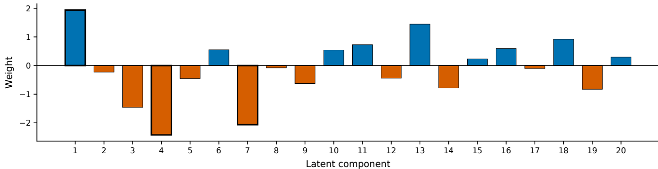
Incident hypertension · Log-odds coefficient (class 1 – class 0)
