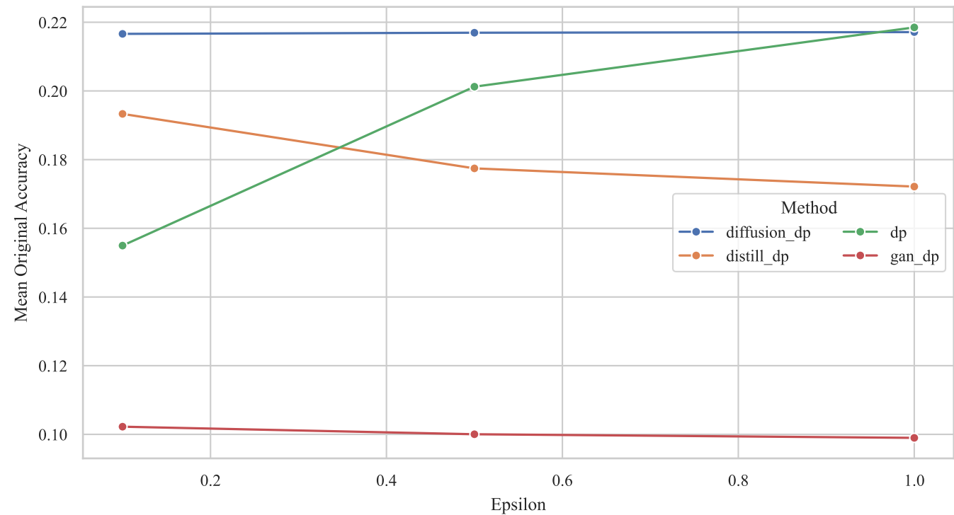
Privacy-Utility Tradeoff (Epsilon vs Accuracy)
