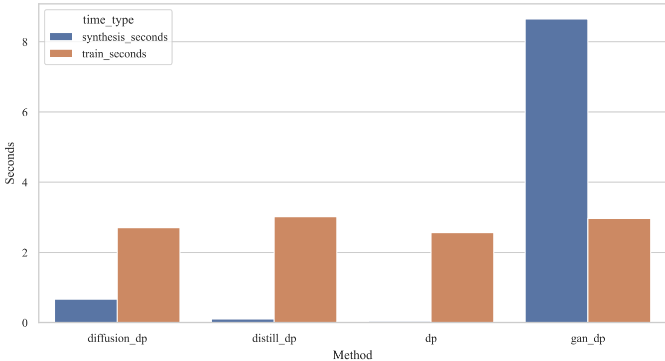
MNIST: Synthesis vs Training Time
