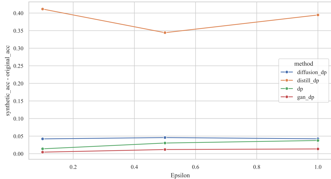
MNIST: Generalization Gap under Epsilon
