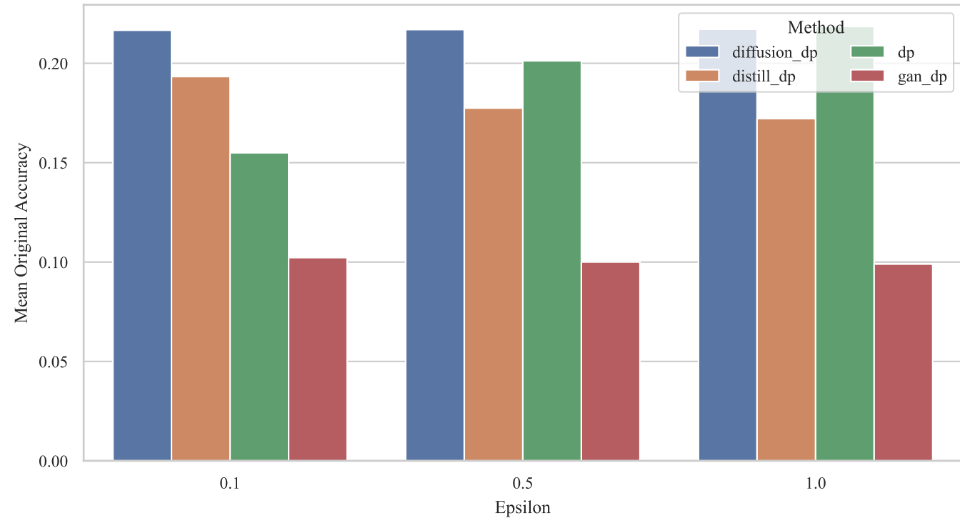
Original Accuracy under Different Privacy Budgets
