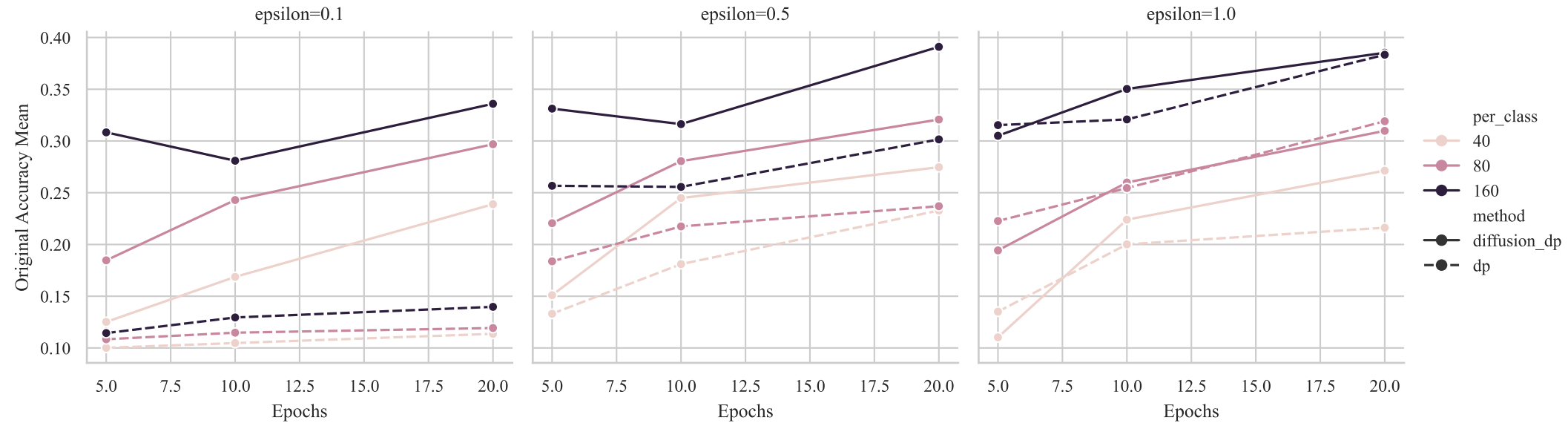
Effect of Training Epochs on Accuracy (ResNet20, k as Color)
