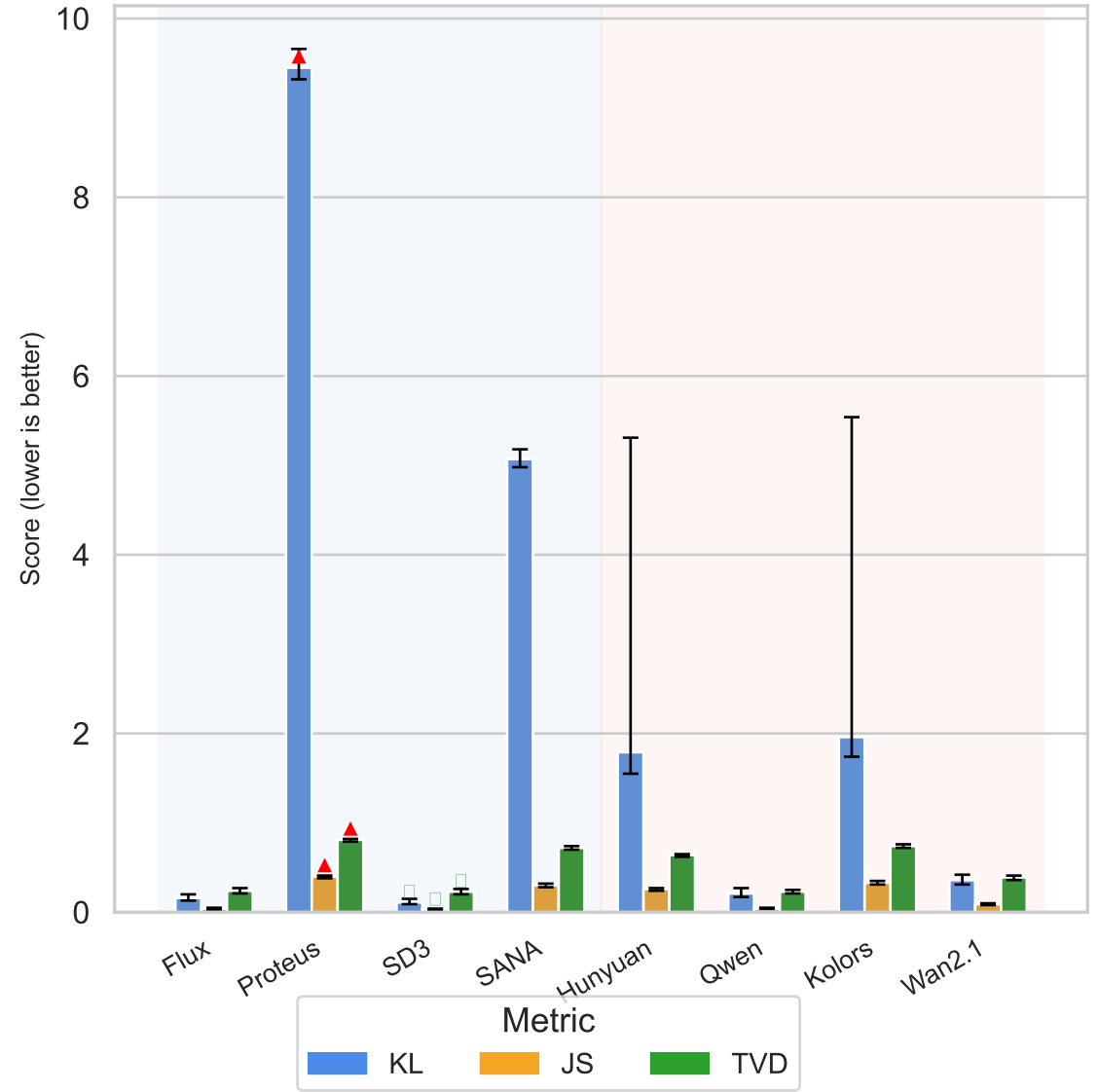
Race
