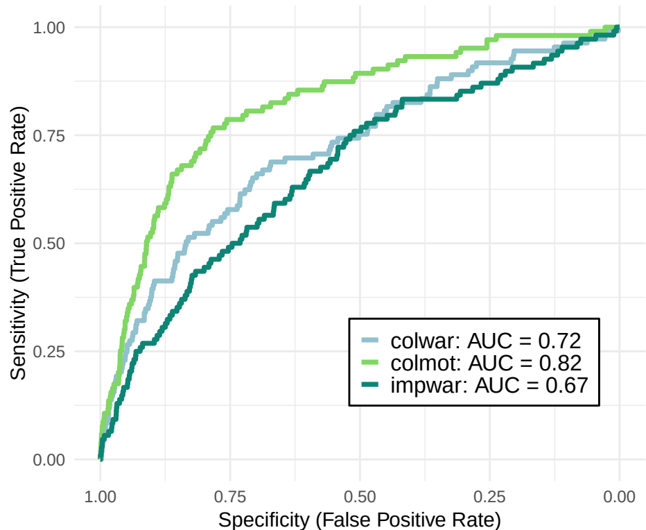
ROC-AUC Plot of War-Decolonization Models
