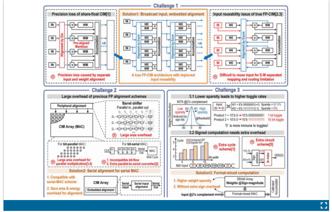
Figure 14.3.1: FP-CIM design challenges and proposed solutions.
