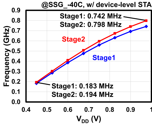
Fig. 10. Performance comparison between MAC stages 1 and 2 with STA.
