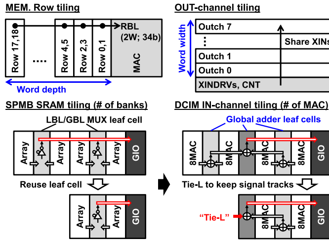
Fig. 14. Tiling method for DCIM compiler; the memory row tiling and the output channel tiling (top), and the input channel tiling (bottom).
