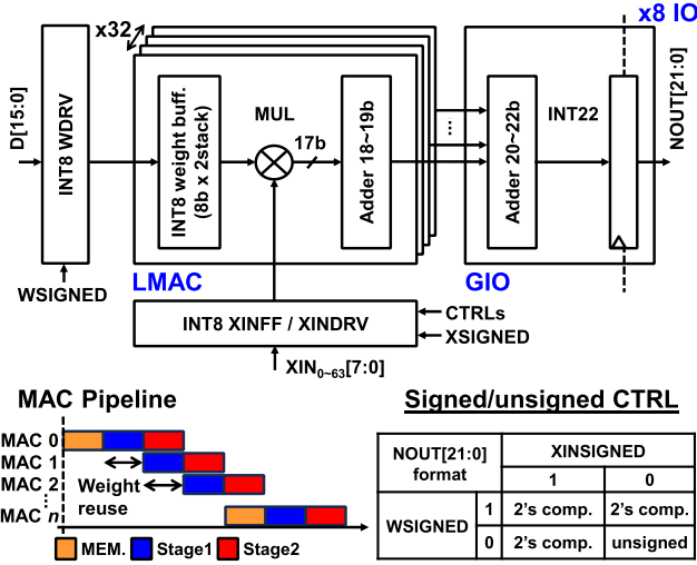
Fig. 6. Architecture overview of INT8 DCIM compiler design (top), Timing diagram of three-stage MAC pipeline and signed and unsigned format handling in INT8 DCIM (bottom).
