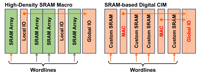
Fig. 1. Concept and floorplan comparison between high-density (HD) SRAM and SRAM-based DCIM.
