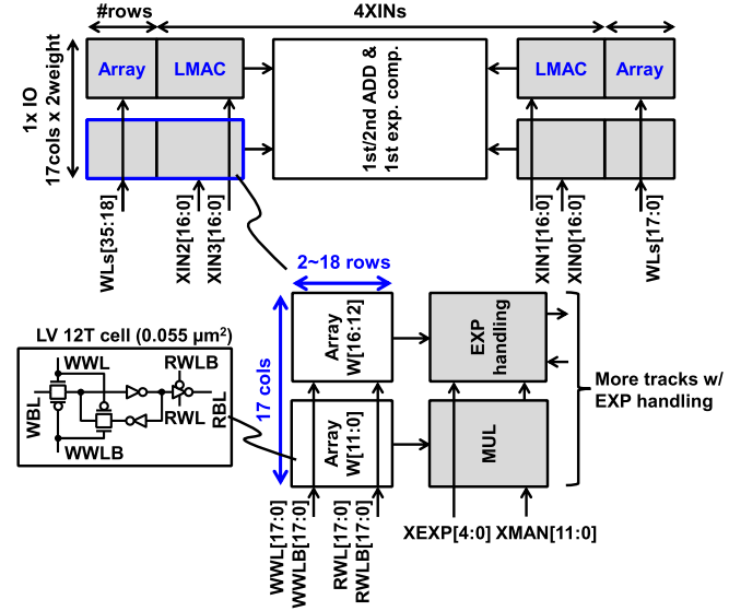
Fig. 8. Layout floorplan for the LMAC with two stacked weight storage and the LV 12 T bitcell schematic.
