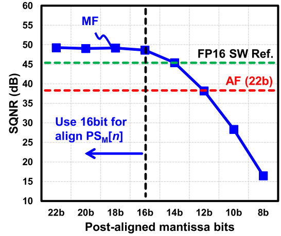
Fig. 5. Arithmetic accuracy based on the SQNR as a function of postaligned mantissa bitwidth.
