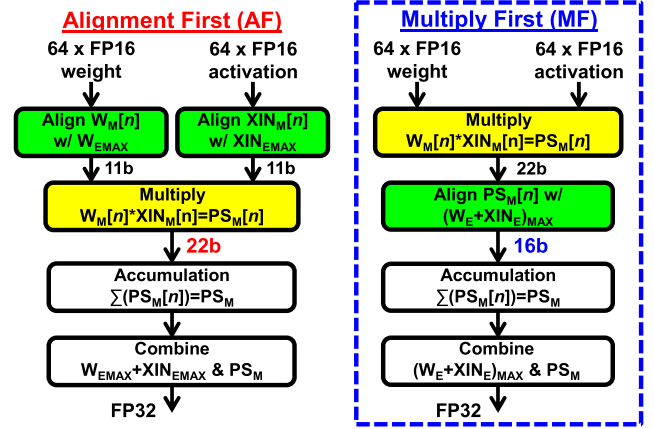
Fig. 4. Comparison of the two common flows of FP processing; the AF approach and the MF approach.
