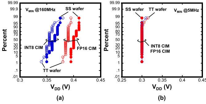
Fig. 16. Measured V_{MIN} . (a) V_{MIN} at testing frequency of 160 MHz and (b) V_{MIN} at testing frequency of 5 MHz.
