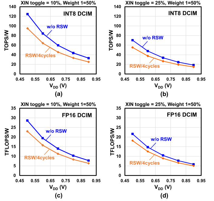
Fig. 18. Power comparison with voltage sweep, different XIN toggle rate, and different memory row switch frequency (RSW). (a) and (b) INT8 DCIM with XIN toggle = 10% and 25% and (c) and (d) FP16 DCIM with XIN toggle = 10% and 25%.
