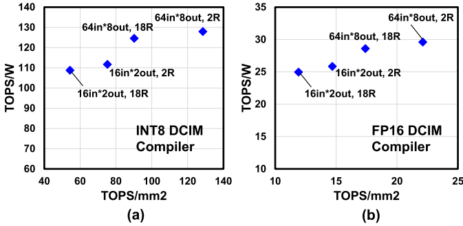
Fig. 20. PPA with different configurations. (a) INT8 DCIM compiler and (b) FP16 DCIM compiler.
