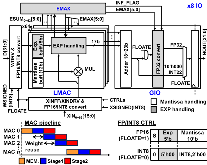
Fig. 7. Architecture overview of FP16/INT8 DCIM compiler design; exponent handling parts are newly adopted (top), timing diagram of three-stage MAC pipeline and FP16 and INT8 modes handling (bottom).
