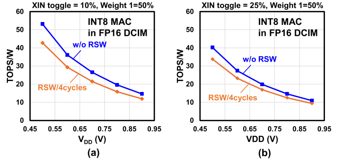
Fig. 19. Power comparison for INT8 MAC mode in FP16 DCIM. (a) XIN toggle = 10% and (b) XIN toggle = 25%.
