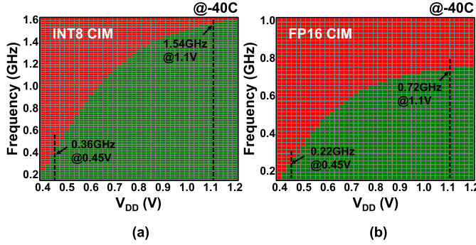
Fig. 17. Measured shmoo plot and f_{MAX} . (a) f_{MAX} for INT8 DCIM and (b) f_{MAX} for FP16 DCIM.
