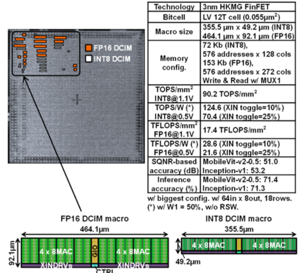
Fig. 15. Test chip micrograph alongside the layout plot and the specification table.
