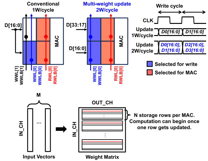
Fig. 11. Conceptual and timing diagram of the multi-weight update per cycle (top) and weight update data flow (bottom).
