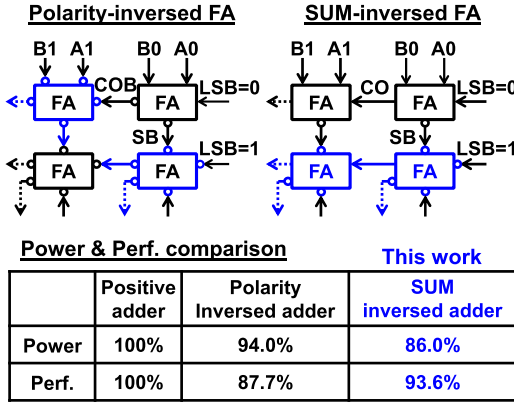
Fig. 13. Power and performance comparison between proposed SUM-inversed FA and conventional polarity-inversed FA.
