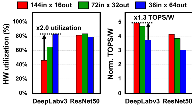
Fig. 3. Impact of macro dimensions on HW utilization and energy efficiency, TOPS/W.
