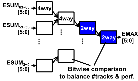
Fig. 9. Maximum exponent (EMAX) search with hierarchical and bitwise comparators.
