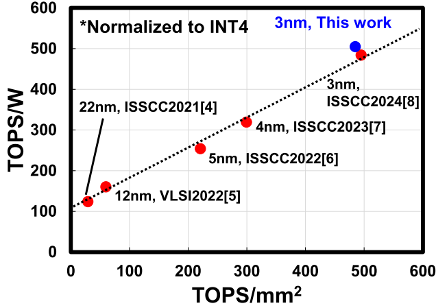
Fig. 2. Normalized TOPS/W and TOPS/mm 2 with technology scaling from 22 to 3 nm.
