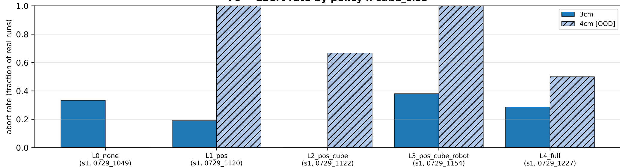
F9 -- abort rate by policy x cube_size
