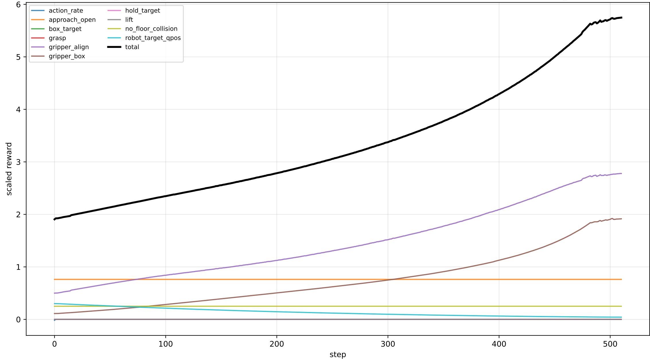
EP200_AS0.025_78fd8855a6eeb72d8ef1a0395cd6e4860db1439d — real run reward (external_stop)
