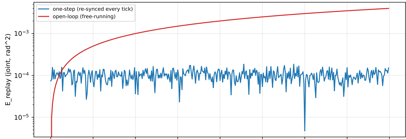
F6 -- dynamics-replay error vs. step (Aljalbout Sec. 5.1 style; time-to-divergence NOT standard terminology -- defined in ur3_dynamics_replay.py)
