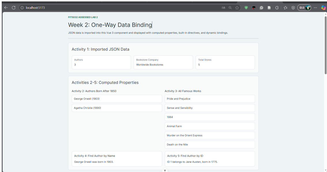
Figure 2: Upper section of the completed Vue.js application for Activities 1–13.
