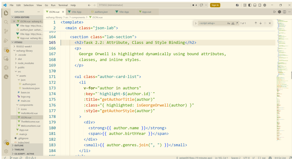
Figure 8: Source code implementing the George Orwell highlight functionality.
