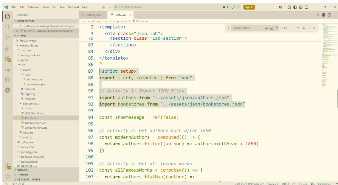
Figure 1: The project structure and JSON imports used for Activity 1.
