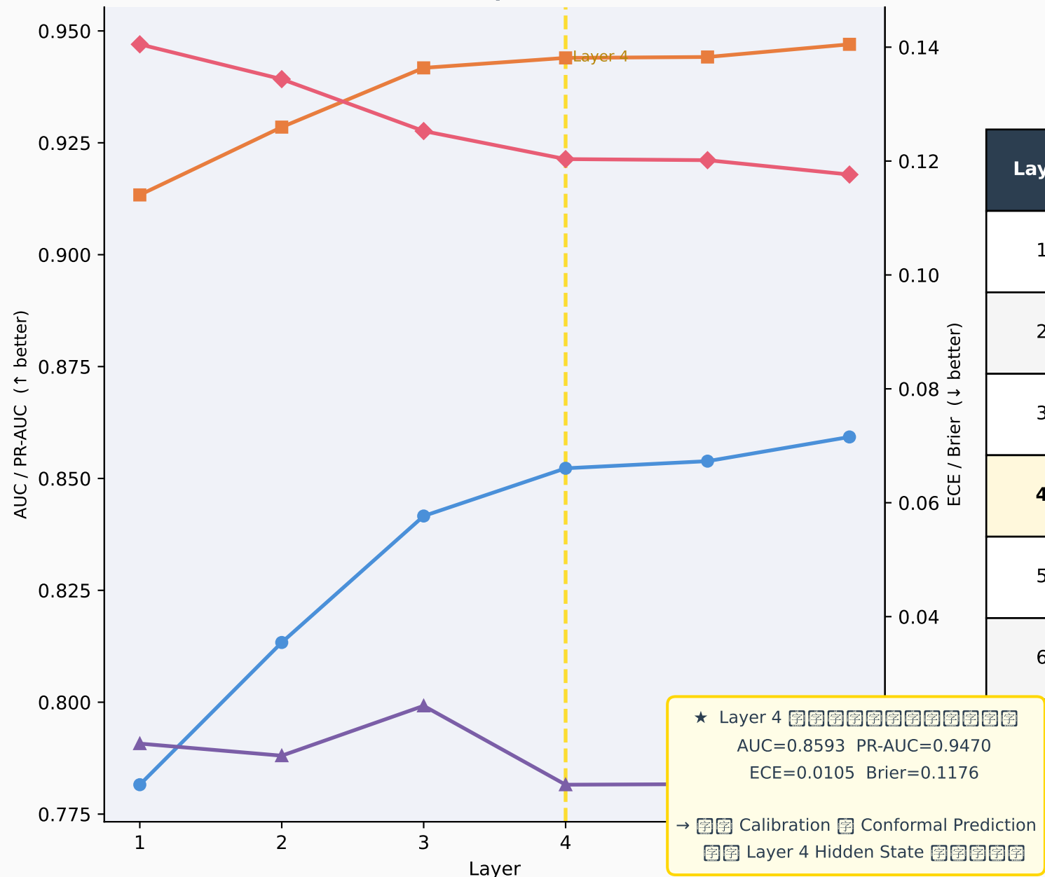
Metric Trends across Layers (Y2 · LGB · split · TEST2)
