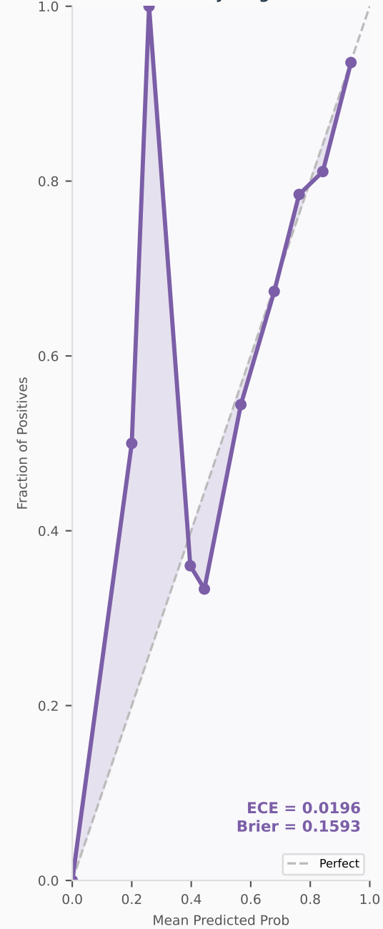
Reliability Diagram
