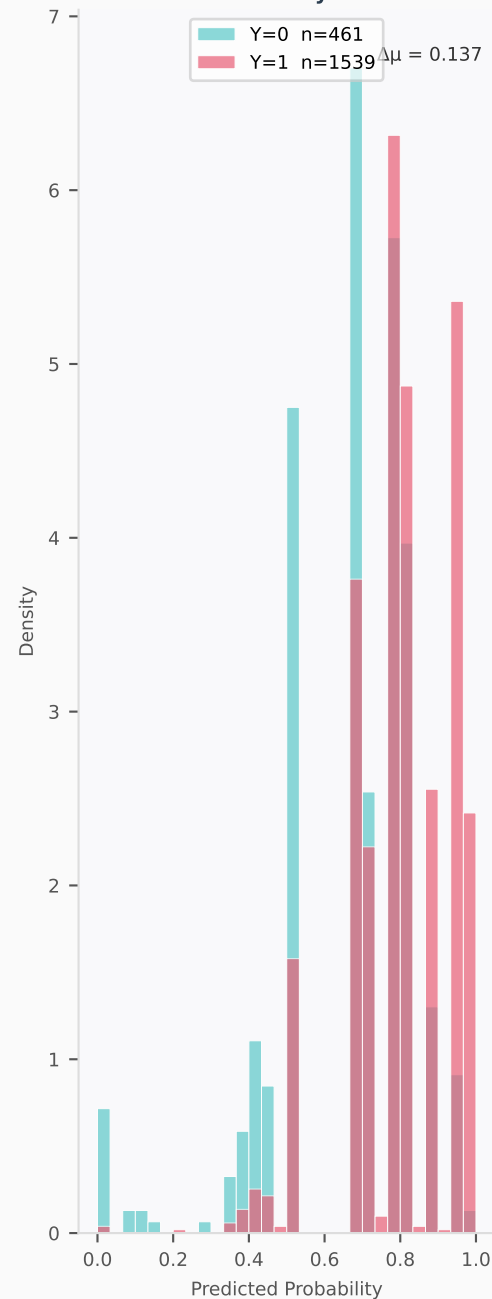
Predicted Prob by True Label
