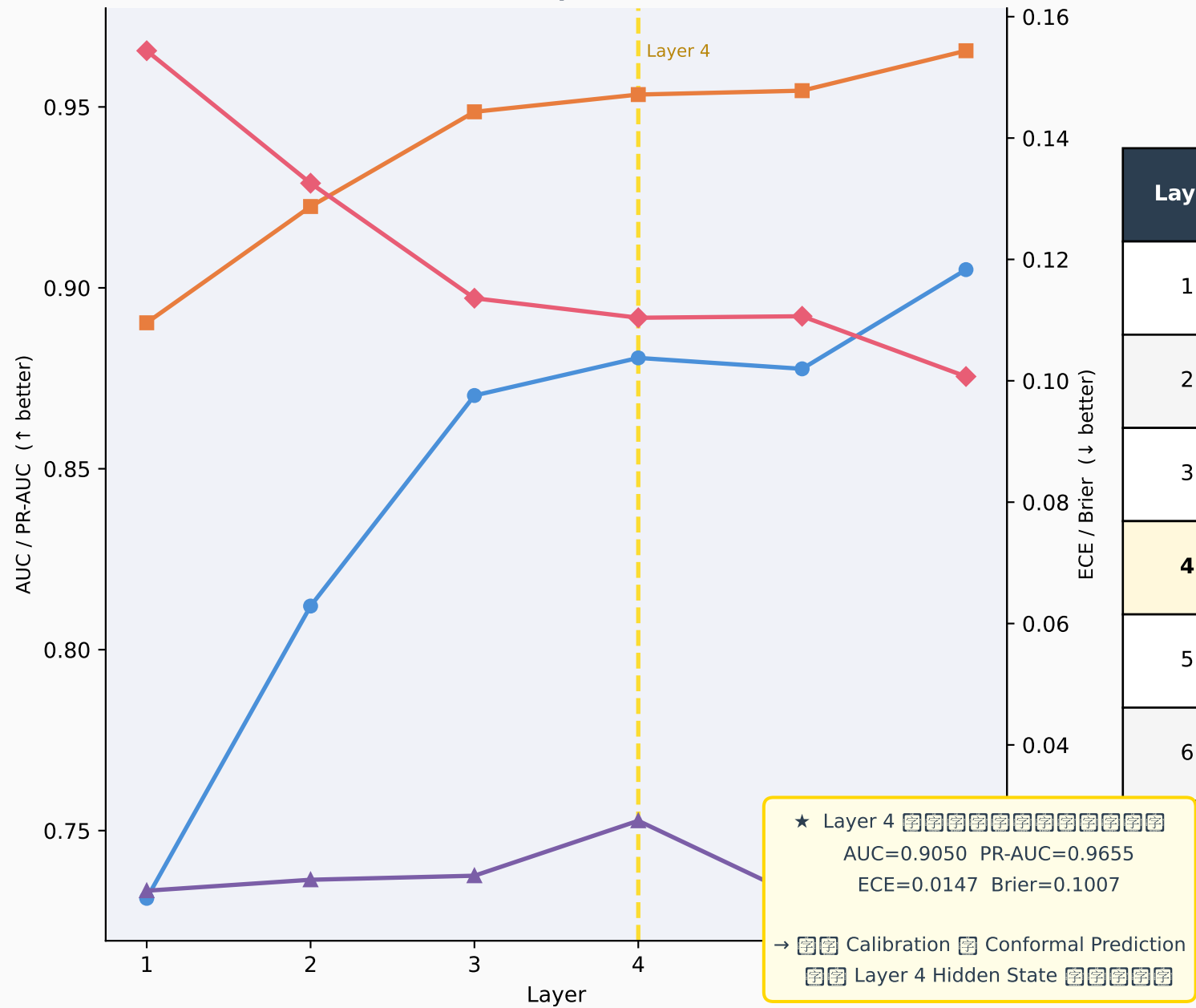
Metric Trends across Layers (Y2 · MLP · split · TEST2)
