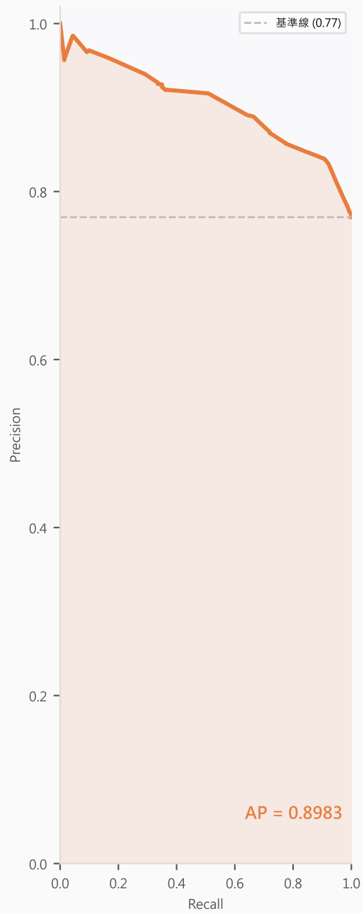
PR Curve
