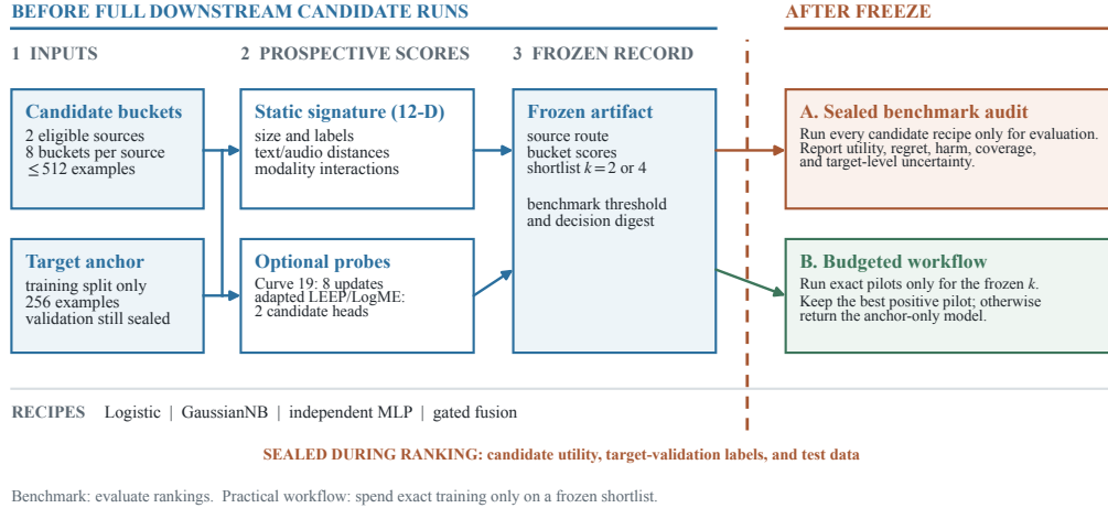
Figure 1: Information boundary and evaluation flow. Candidate buckets and target training anchors are used to compute prospective scores. The route, ranking, rejection threshold, and shortlist are recorded before candidate utility or validation labels are accessed. The benchmark then trains every candidate for audit. The budgeted procedure evaluates only the frozen shortlist and keeps either the best positive pilot or the anchor-only model.
