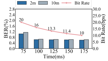
Figure 23: Transmission Capacity.
