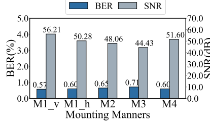
Figure 22: HDD mounting manners.
