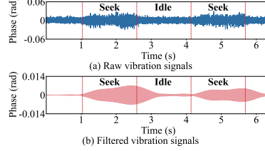
Figure 6: Model of the HDD vibration. Figure 7: Raw and filtered vibrations.
