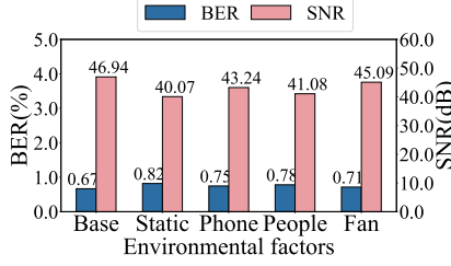
Figure 21: Environmental factors.
