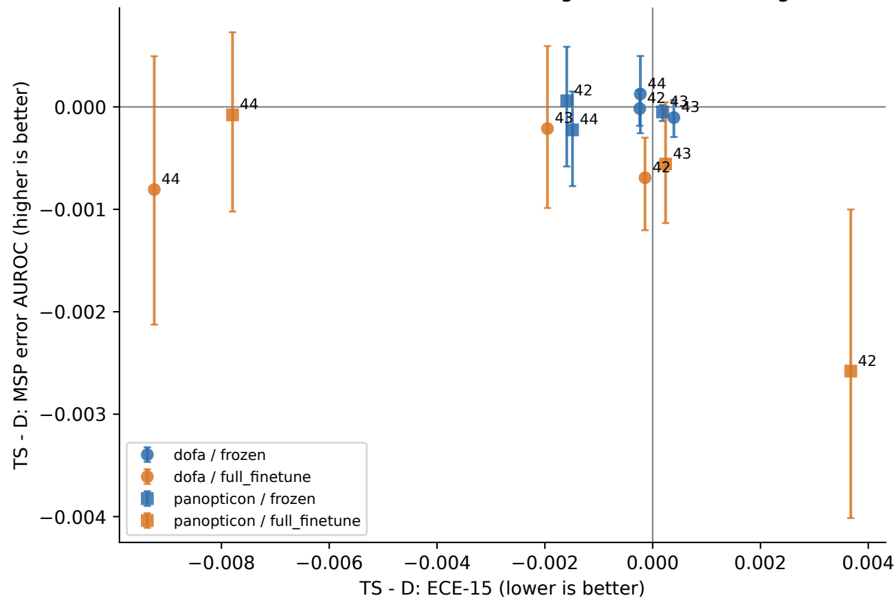
EuroSAT: calibration and error ranking need not move together
