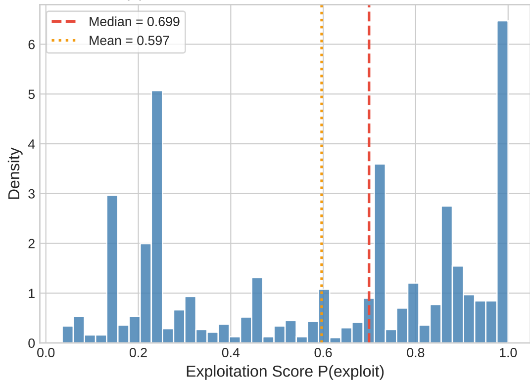
(b) Snorkel Label Model Score Distribution
