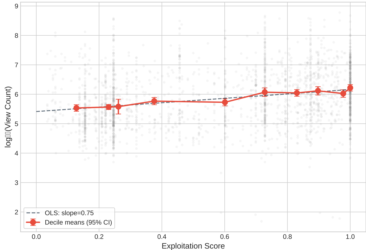
Exploitation Score vs. Video Popularity (Spearman \rho = 0.270 , p < 10^{-3} , n = 2,305 )
