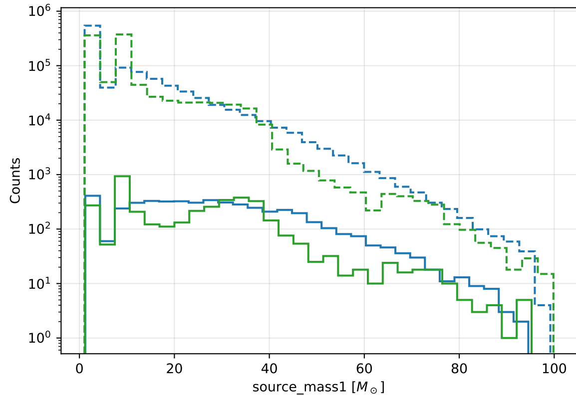
GWTC-3 vs GWTC-4: Source mass1
