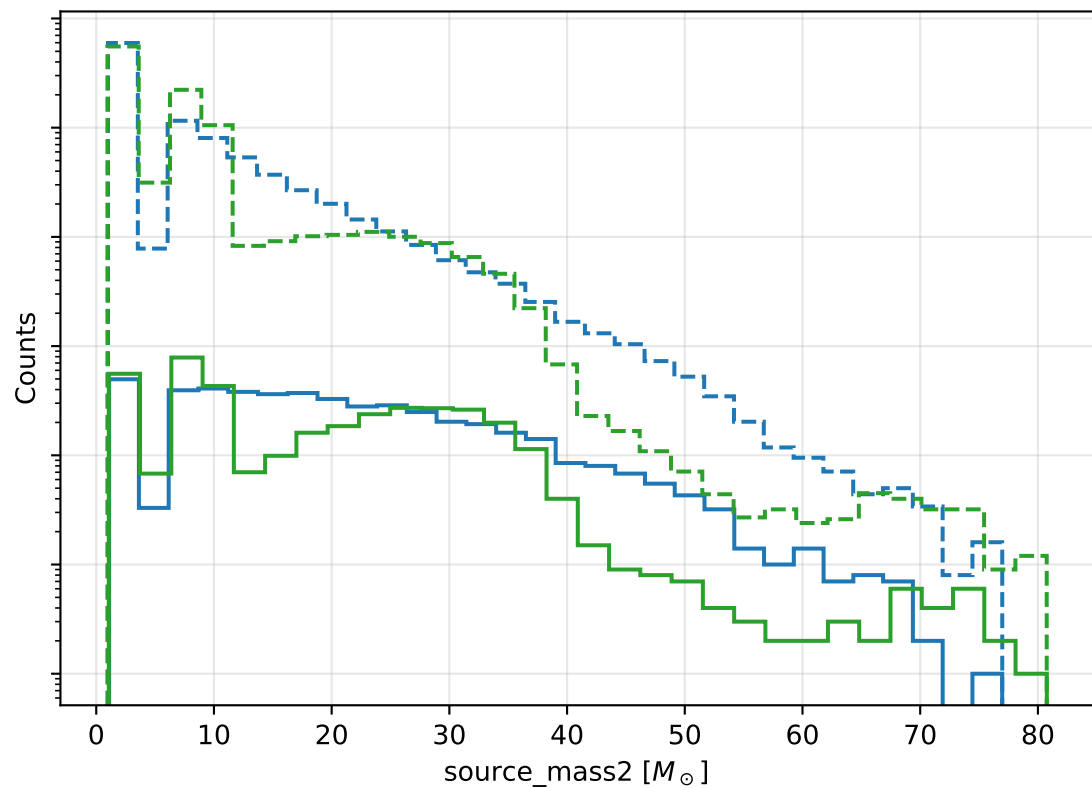
GWTC-3 vs GWTC-4: Source mass2
